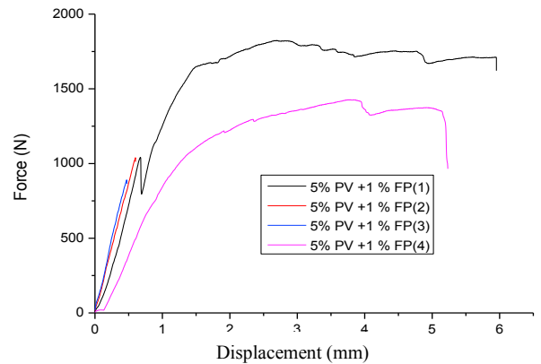
Fig 8: Three point flexural curve test results (Composition 4).
