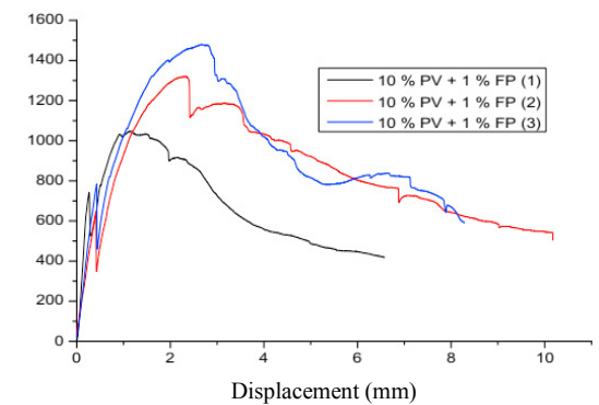
Fig 10: Three point flexural curve test results (Composition 6).
