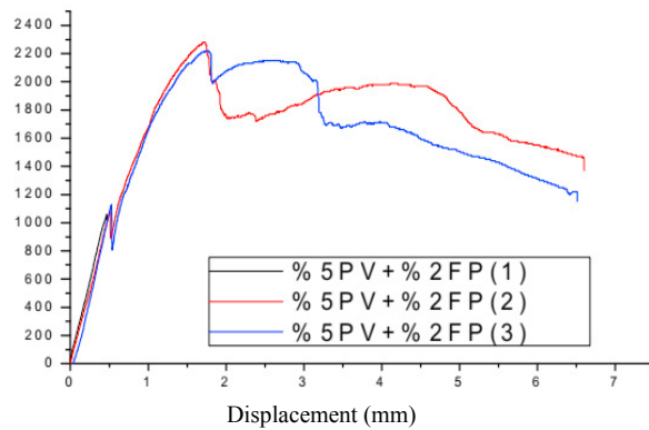
Fig 9: Three point flexural curve test results (Composition 5).
