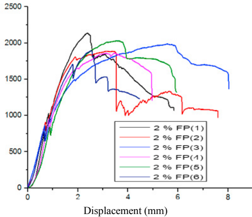
Fig 7 Three point flexural curve test results (Composition 3).
