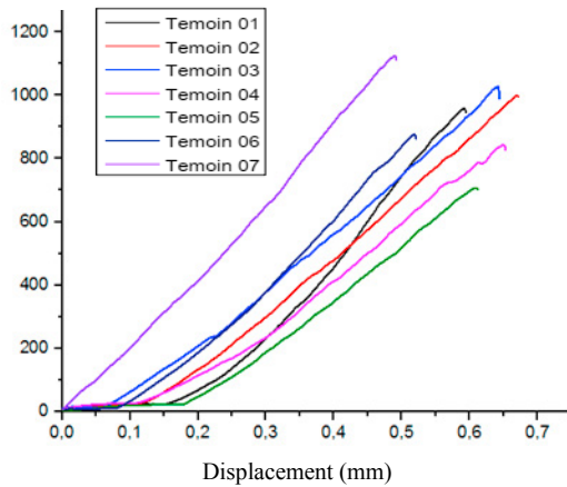
Fig 5: Three point flexural curve test results (Composition 1).
