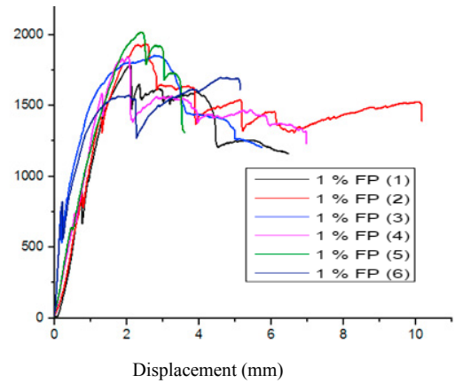
Fig 6: Three point flexural curve test results (Composition 2).
