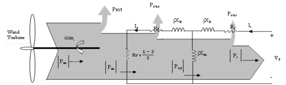
Figure 4. Power flow and losses in an IG.
