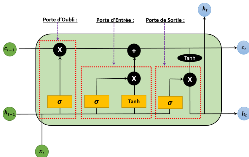
FIGURE 4.5 – LSTM Architecture [ Basé sur [48] ]
