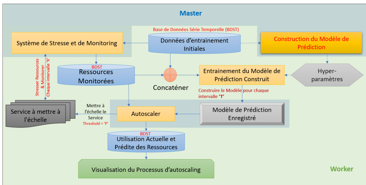
FIGURE 6.1 – Architecture Globale de MEAP
