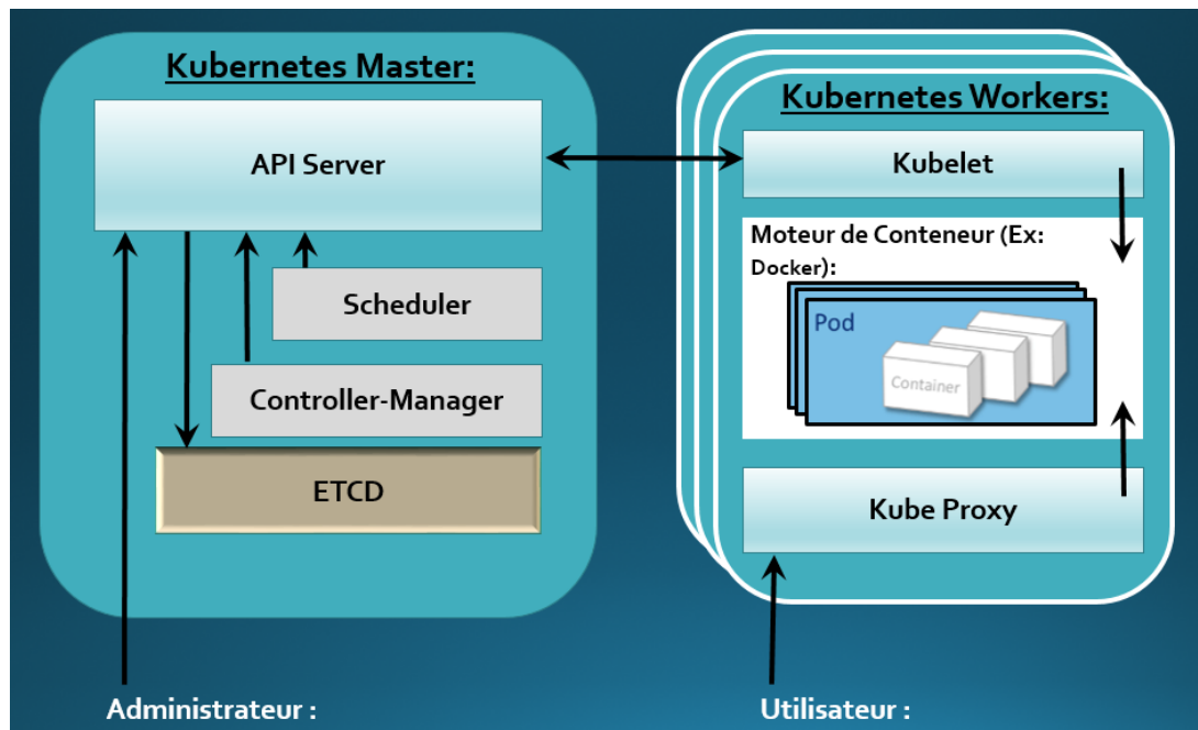
FIGURE 3.1 – Architecture de Kubernetes [ Basé sur[9] ]
