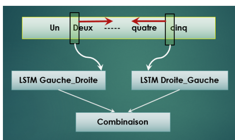
FIGURE 4.18 – LSTM Bidirectionnels [ Basé sur [13] ]
