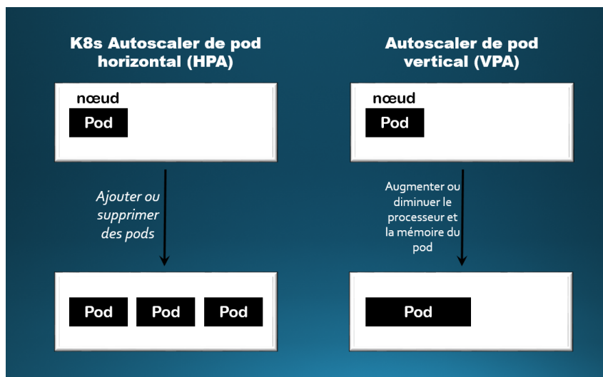
FIGURE 3.5 – HPA VS VPA [ Basé sur [77] ]
