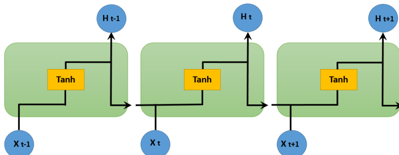
FIGURE 4.3 – Tanh [ Basé sur [6] ]
