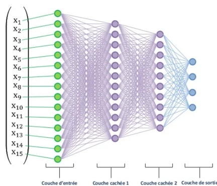
FIGURE 4.1 – Architecture des ANN [6]
