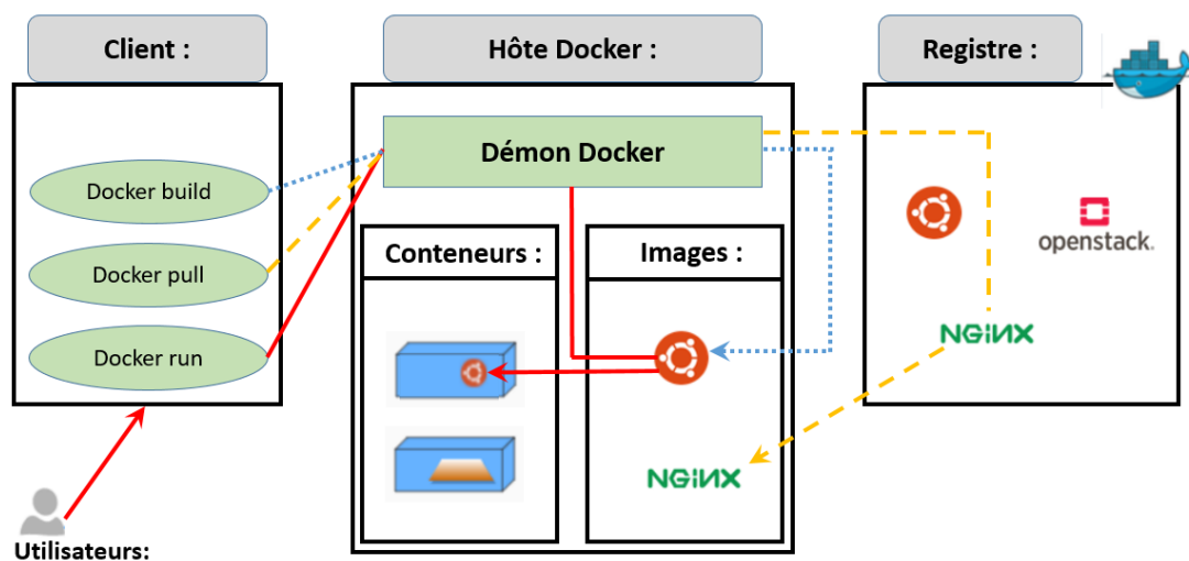
FIGURE 2.1 – Architecture de Docker [ Basé sur [8] ]
