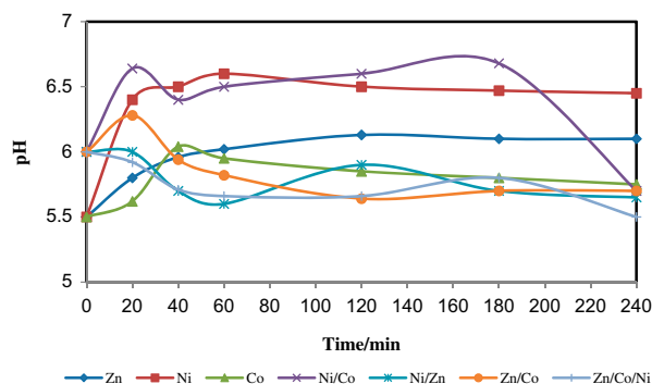
Fig. 4. The variation in the pH values of modified bentonite suspensions as a function of time.
