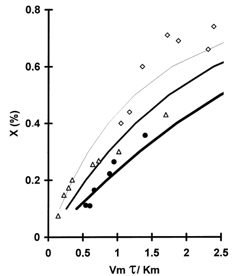
Fig. 8. Course of fractional conversion ( X ) against V_m \tau / K_m . Experimental data ( \bullet ) S_0 = 37.5 \text{ g dm}^{-3} , ( \Delta ) S_0 = 18.8 \text{ g dm}^{-3} and ( \diamond ) S_0 = 4.5 \text{ g dm}^{-3} . Theoretical curve ( \blacksquare ) S_0 = 37.5 \text{ g dm}^{-3} , ( \blacksquare ) S_0 = 18.8 \text{ g dm}^{-3} and ( - ) S_0 = 4.5 \text{ g dm}^{-3} .
