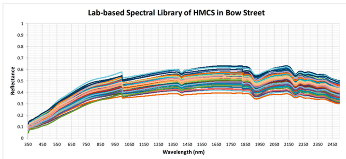
Figure 7. Lab-based spectral library of the heavy metal soil contamination (HMSC) at the Bow Street site.
