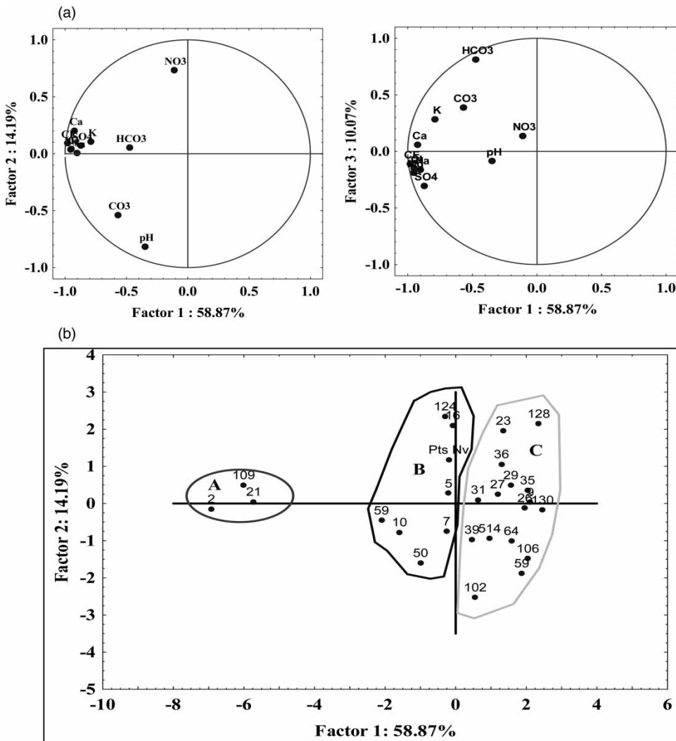
Figure 3 | Results of principal component analysis (PCA). (a) Variables (chemical parameters) graph and (b) individual (observations) graphs.
