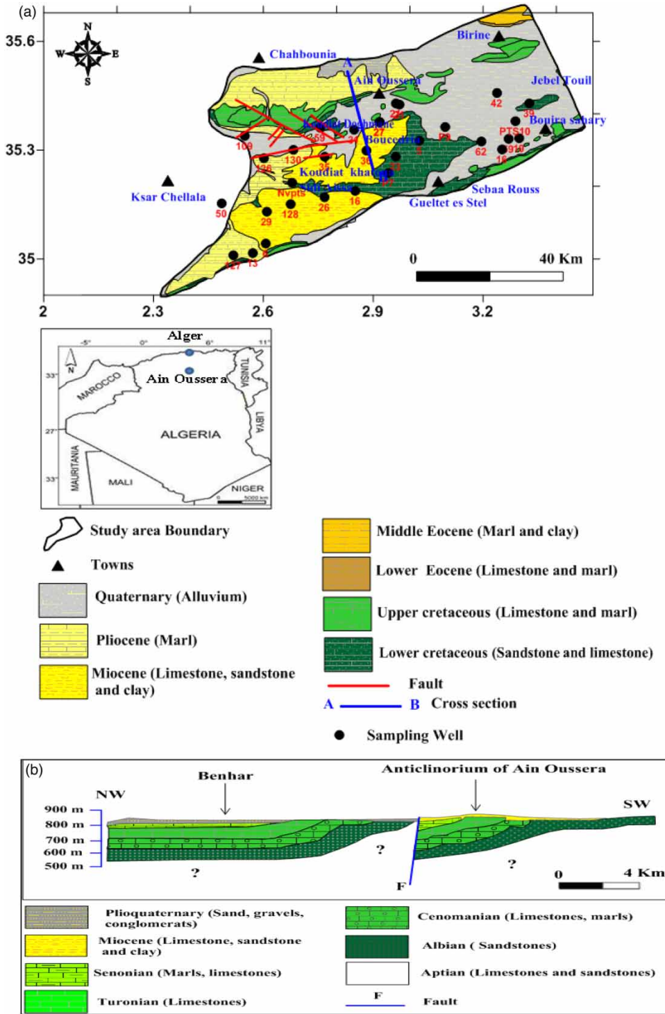
Figure 1 | (a) Geological map of the study area and groundwater sample locations. (b) Synthetic geological cross section, along transect (AB) (Maoui et al. 2013).
