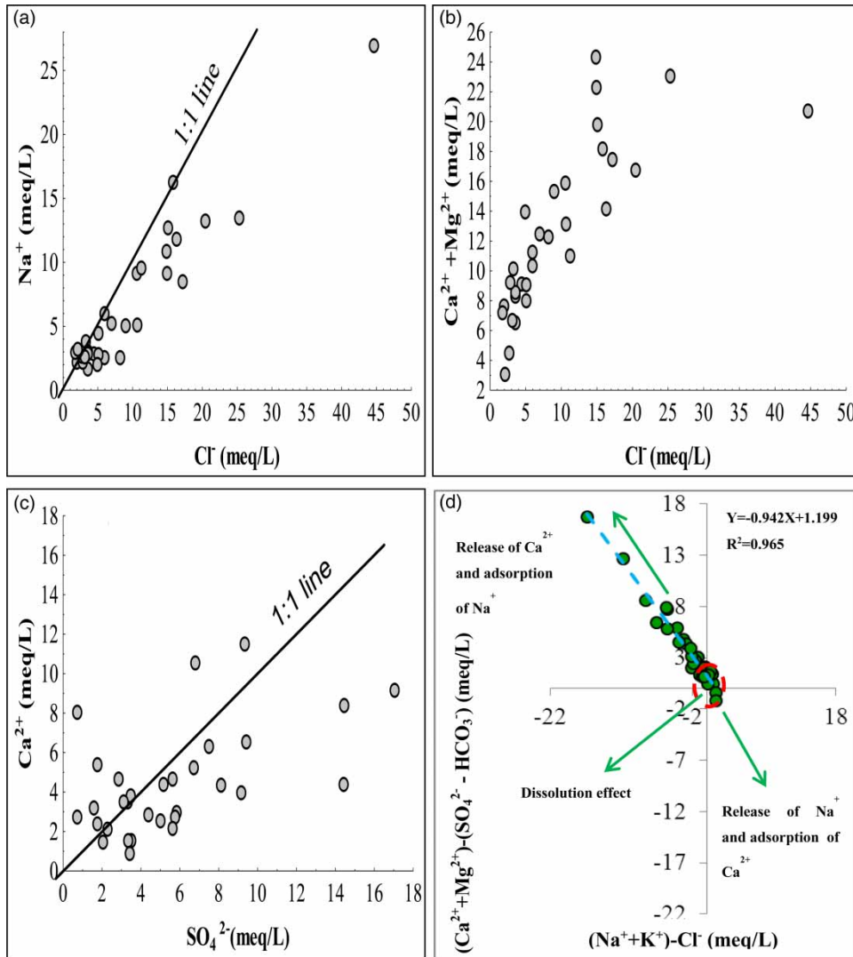
Figure 4 | Relationship between major elements: (a) \text{Na}^+/\text{Cl}^- , (b) \text{Ca}^{2+} + \text{Mg}^{2+}/\text{Cl}^- , (c) \text{Ca}^{2+}/\text{SO}_4^{2-} , (d) [(\text{Ca}^{2+} + \text{Mg}^{2+}) - (\text{HCO}_3^- + \text{SO}_4^{2-})]/(\text{Na}^+ + \text{K}^+) - \text{Cl}^- .
