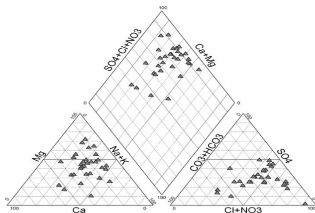
Figure 2 | Piper diagram of groundwater samples.
