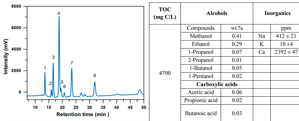
Fig. 1. On the left, HPLC chromatograms of the Fischer-Tropsch product water (1: acetic acid 2: propionic acid 3: methanol 4: ethanol 5: butanoic acid 6: 2-propanol 7:1-propanol 8: butanol); on the right, quantification of the main organic and inorganic compounds.
