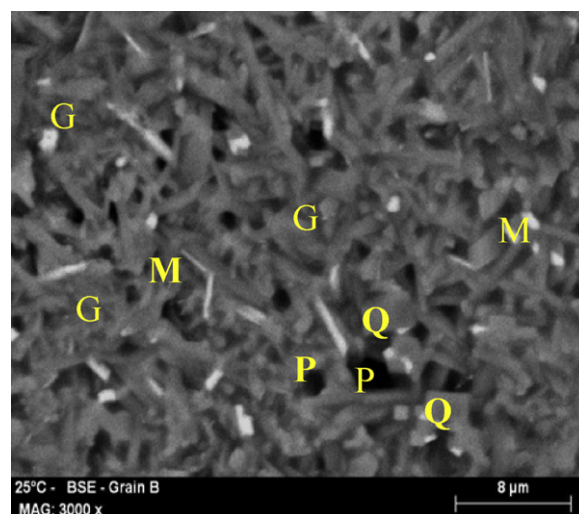
Fig. 5. SEM micrograph of a BSAA refractory brick (hallohsite and KT kaolin brick) fired at 1350 °C (M: Mullite needles; Q: Quartz; G: Amorphous phase; P: Pores).
